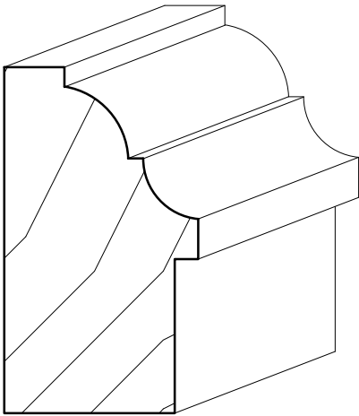
BB-4 2" X 1 1/8"
