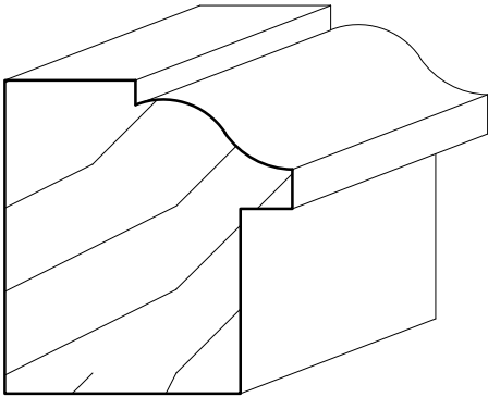
BB-13 1 1/2" X 1 3/8"
