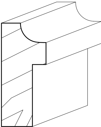
BB-16 3/4" X 1 3/4"
