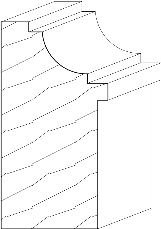
BB-15 1 7/8" X 3 5/8"
