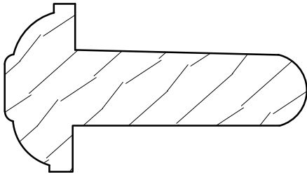
T-AST-1 1 \frac{1}{4}'' \times 2 \frac{1}{4}'' FOR 1 \frac{3}{4}'' DOOR
