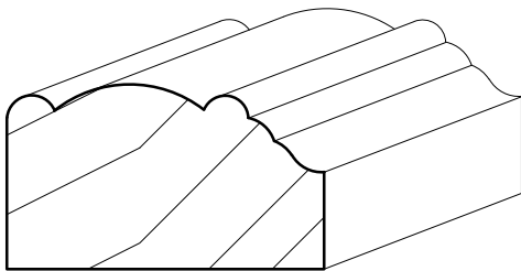
D-12 7/8" X 1 1/2"
