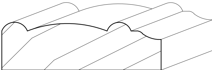
D-14 7/8" X 2 7/8"
