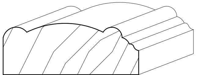
D-13 7/8" X 2 5/16"
