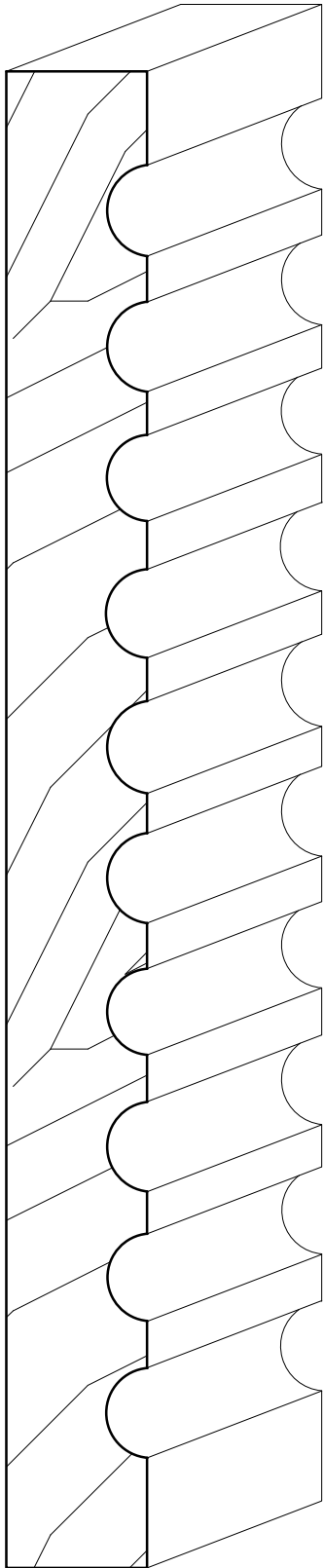
FLUTED-4 \frac{3}{4}'' \times 8''
